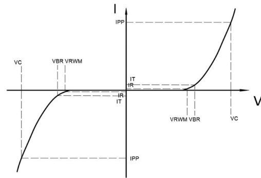
V-I characteristics for a Bi-directional TVS
